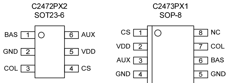
Figure 2: C2472 and C2473 Pin Assignment (drawings are not to scale)
