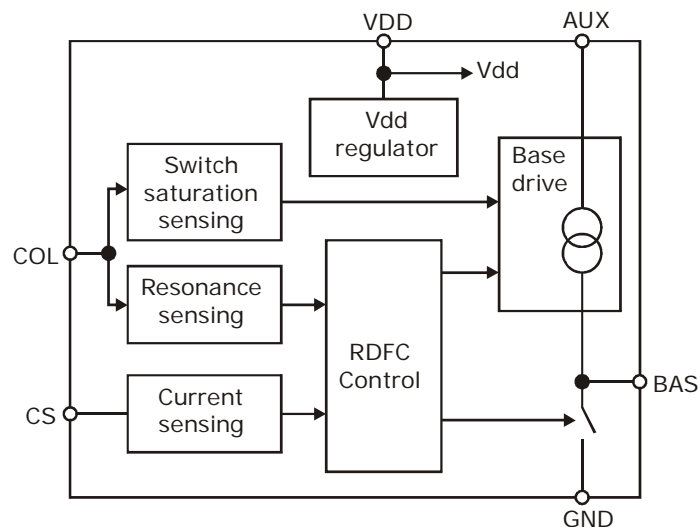
Figure 1: Block Diagram of the C2472 and C2473 Controller ICs
