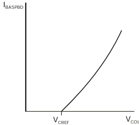
Figure 9: I_{BASPBD} characteristic
